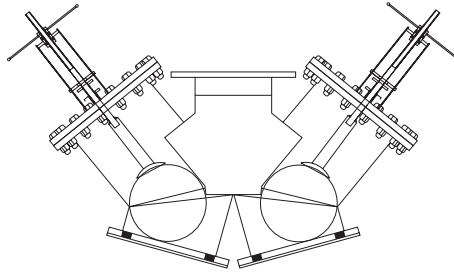
Both Pumps Isolated. With Handwheels. No Flow.
